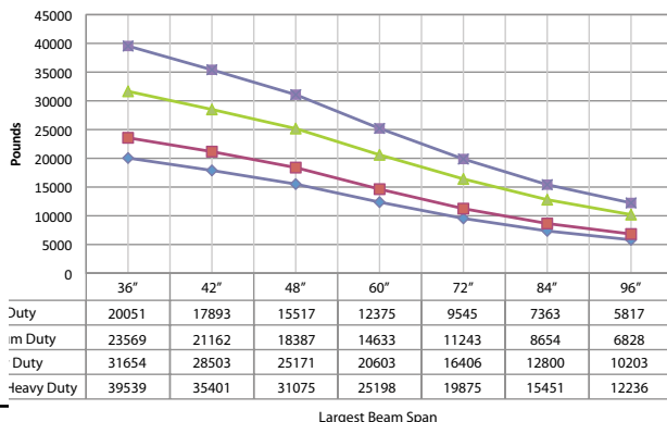
Upright Capacity Chart
