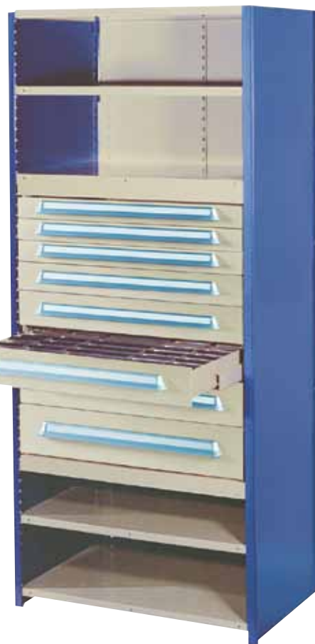
Modular drawer installation should have a shelf directly above and below the drawer guide support as shown.
