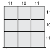
C - 9 compartments
