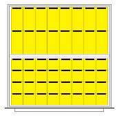
BA - 48 plastic bins 3" w x 3" d, 3" w x 3" d & partition
